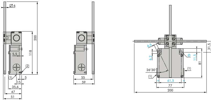
XCKWMR54D1H29 / XCKWMR54D2H29
