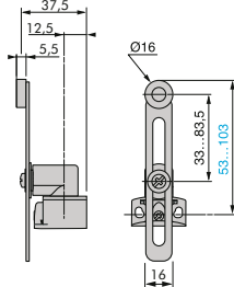
ZCE01 + ZCY45
