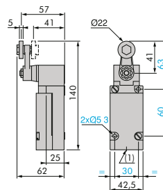
XCKWJ210513H29 XCKWJ210511H29
