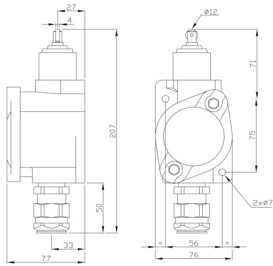
XC8-JC162P1...
