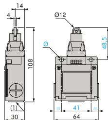
XCKWM2102H29
