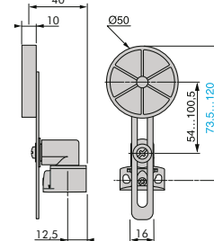
ZCE01 + ZCY49
