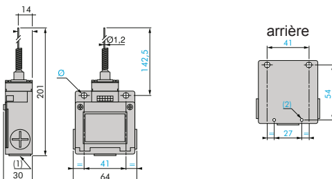
XCKWM2106H29
